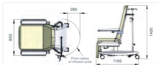
Flawless technology even in very enclosed spaces (measurements in mm)
